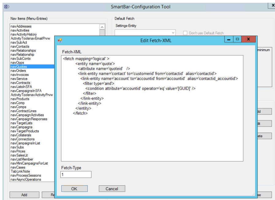
Figure 15: Edit fetch
