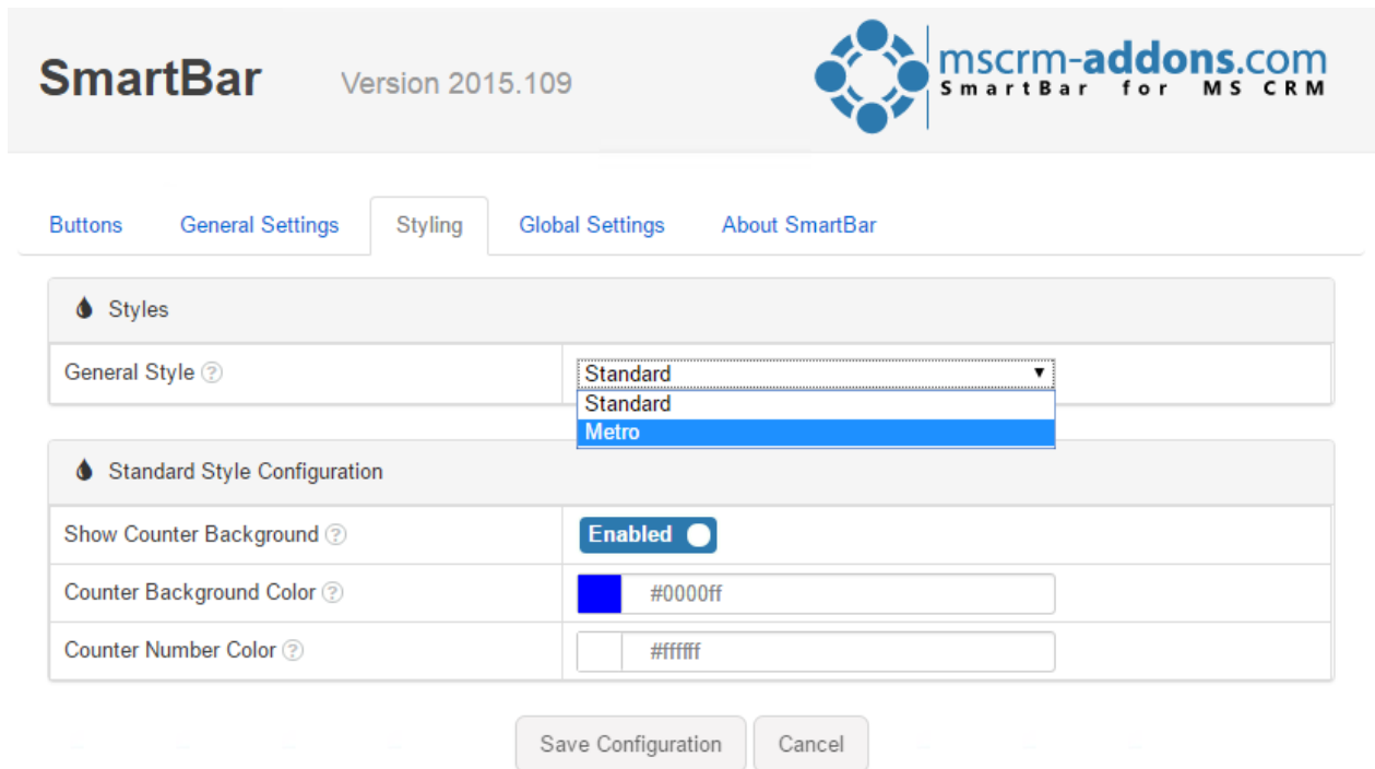
Figure 28: SmartBar – Styling-tab
